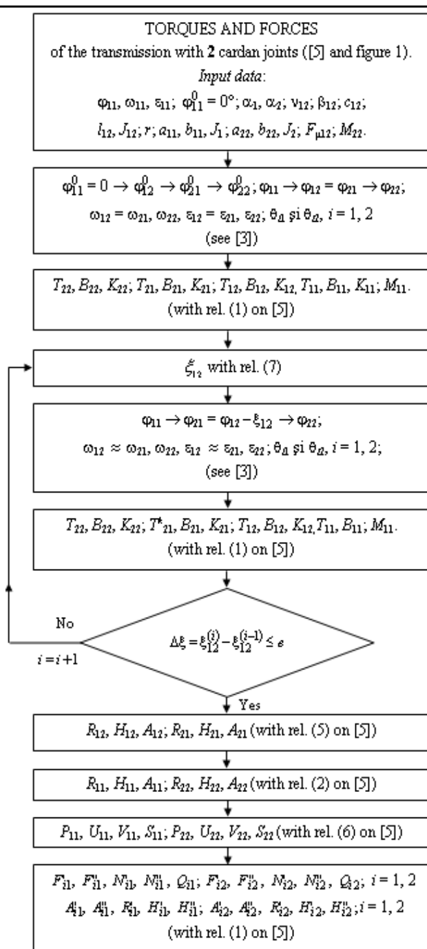
Fig. 2. Flow chart of the modular modeling algorithm of a 2-cardan transmission, considering the secondary shaft elastic
