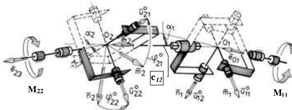
Fig. 1. Variantă de transmisie bicardanică determinată static, cu arbore intermediar elastic Fig. 1. Version of a statically determined 2-cardan transmission, with elastic secondary shaft
