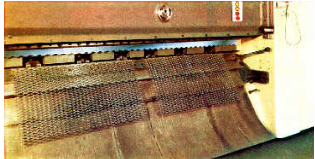
Figure 3. The working area and the mobile cutter of a sheet metal expanding machine
