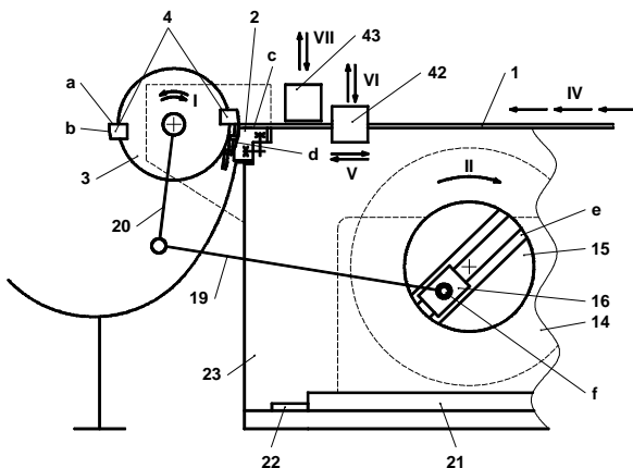
Figure 6. The kinematic diagram of a sheet metal expanding machine with oscillatory main motion (side „view”; detail)
