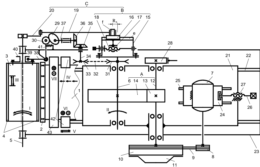
Figure 5. The kinematic diagram of a sheet metal expanding machine with oscillatory main motion (including shaft axes)
