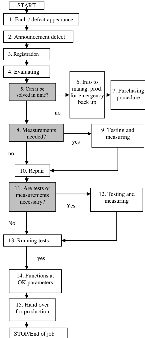
Figure 3. Maintenance procedure
